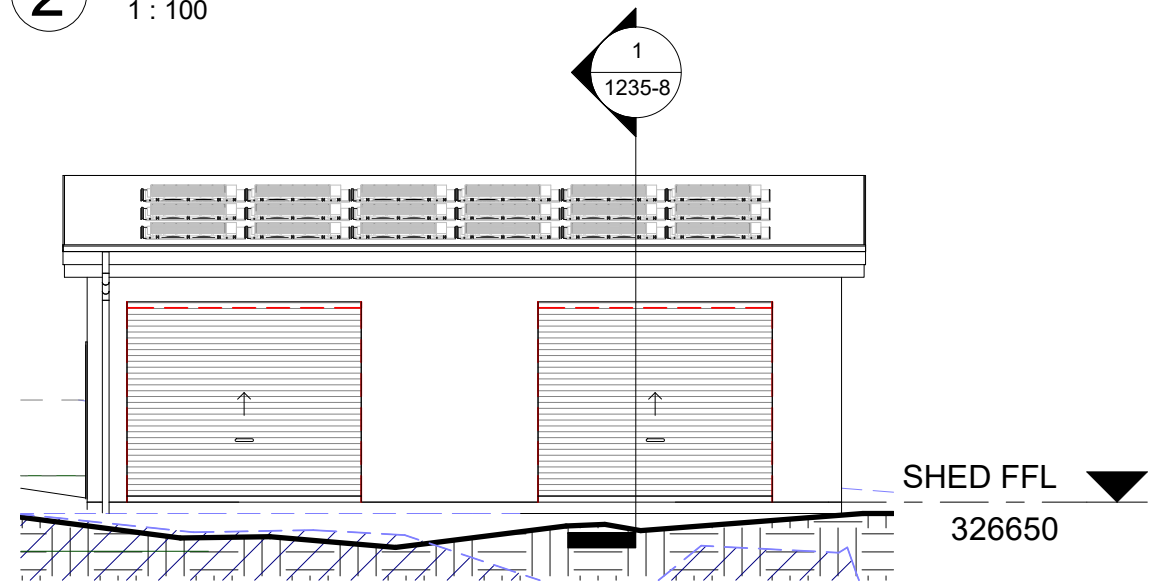
2 SHED SOUTH ELEVATION 1 : 100
