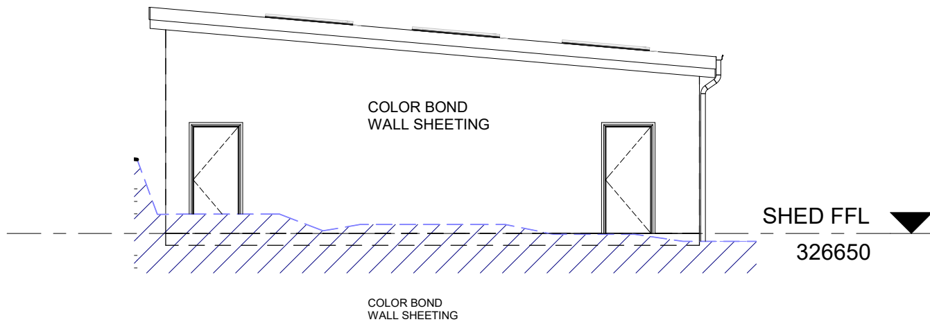
3 SHED EAST ELEVATION 1 : 100
