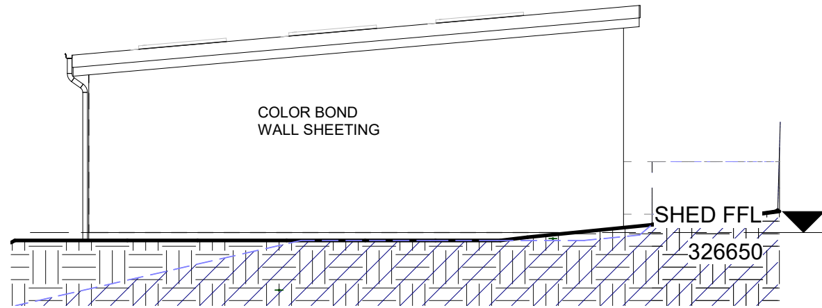
1 SHED WEST ELEVATION 1 : 100
